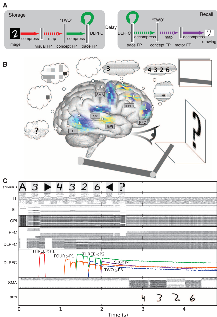
Fig. 2. The serial WM task. (A) Information flow through Spaun during the WM task. Line style and color indicate the element of the functional architecture in Fig. 1B responsible for that function. FP, firing pattern. (B) A screen capture from the simulation movie of this task (supplementary section S2.1), taken at the 2.5-s mark of the time course plot in (C). The input image is on the right, the output is drawn on the surface below the arm. Spatially organized (neurons with similar tuning are near one another), low-pass-filtered neuron activity is approximately mapped to relevant cortical areas and shown in color (red is high activity, blue is low). Thought bubbles show spike trains, and the results of decoding those spikes are in the overlaid text. For Str, the thought bubble shows decoded utilities of possible actions, and in GPI the selected action is darkest. (C) Time course of a single run of the serial WM task. The stimulus row shows input images. The arm row shows digits drawn by Spaun. Other rows are labeled by their anatomical area. Similarity plots (solid colored lines) show the dot product (i.e., similarity) between the decoded representation from the spike raster plot and concepts in Spaun's vocabulary. These plots provide a conceptual decoding of the spiking activity, but this decoding is not used by the model (supplementary section S1.1). Raster plots in this figure are generated by randomly selecting 2000 neurons from the relevant population and discarding any neurons with a variance of less than 10% over the run. ⊗ denotes the convolution compression operator.
